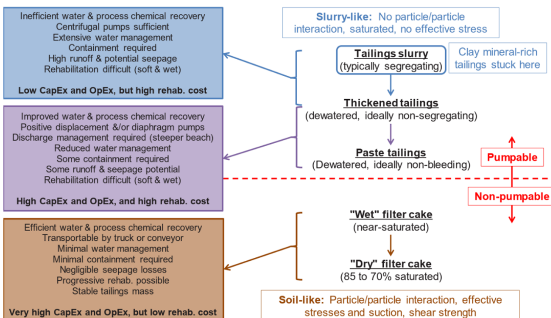
Fig. 5. Benefits and challenges of tailings dewatering technologies. Source: (Davies & Rice, 2001; LPSDP, 2016).
