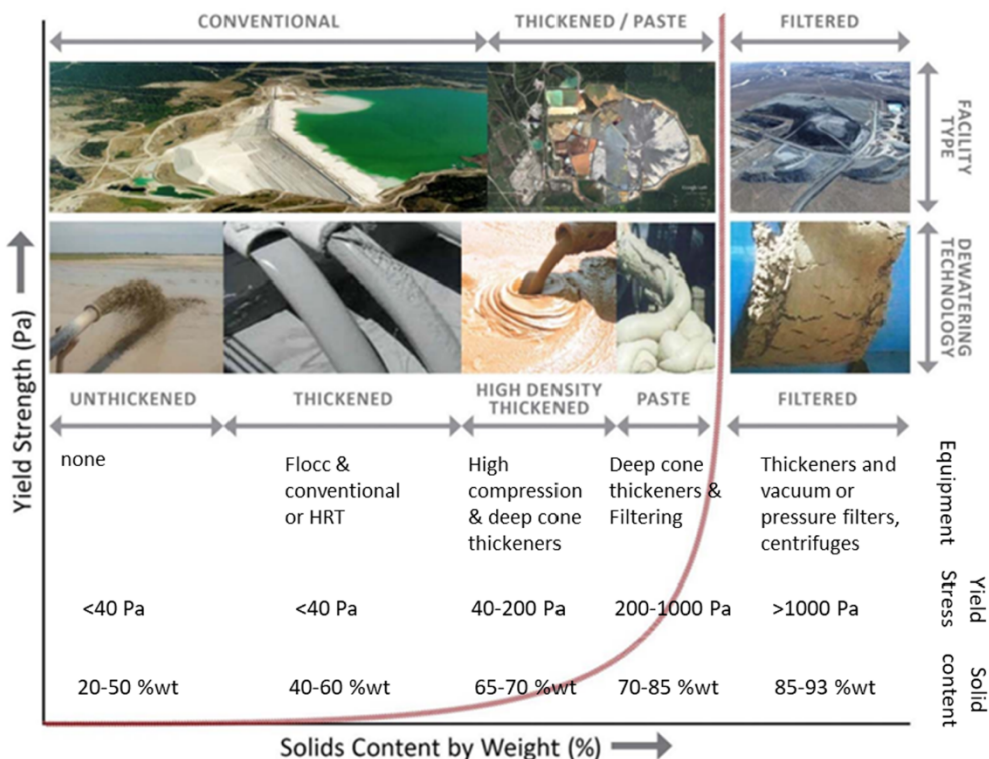
Fig. 4. Range of application for dewatering of tailings. Source: After MEND 2017.
