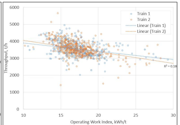
Figure 7 – W_{io} vs. Throughput (RGS)
